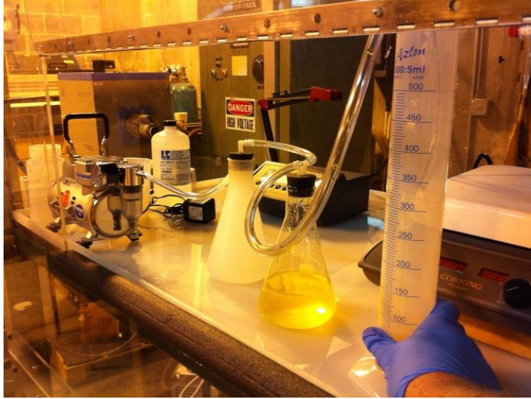
Figure 4.6 – Siphoning off supernate liquid before filtering out \text{Fe}(\text{OH})_3 solids
